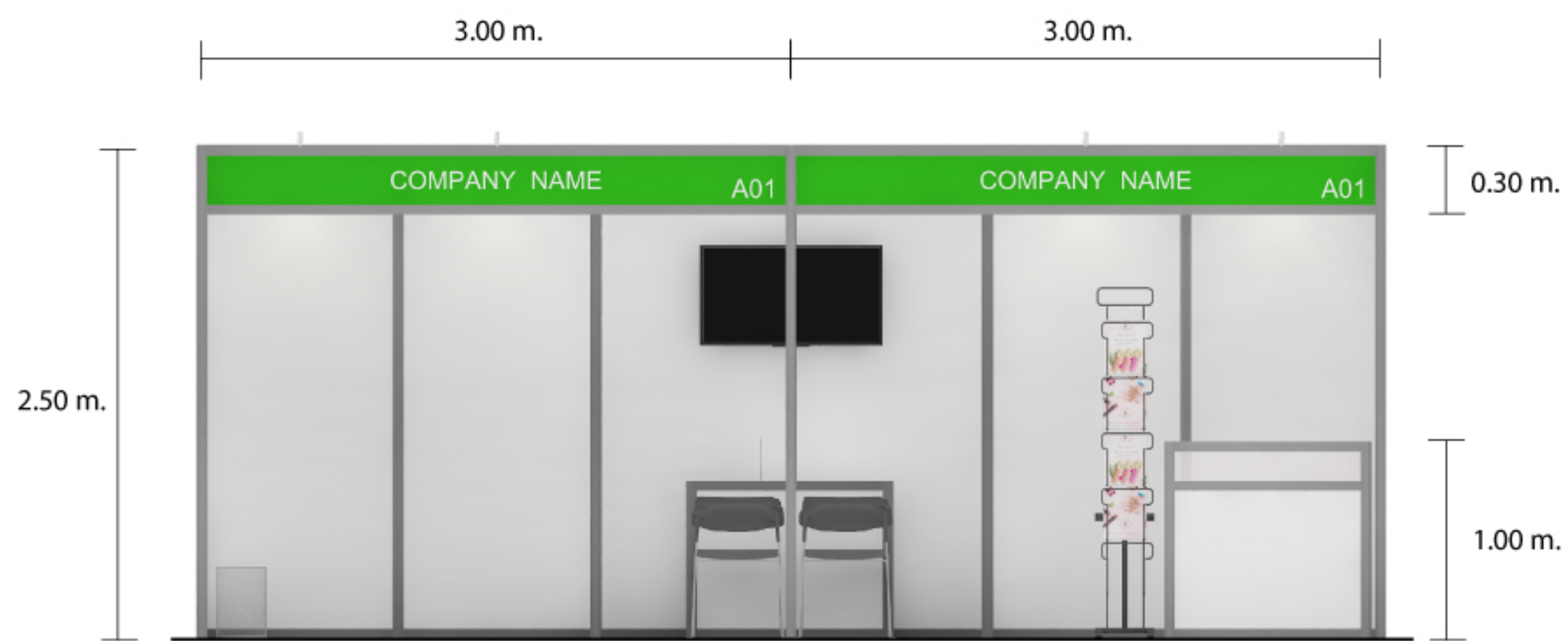
FRONT VIEW
