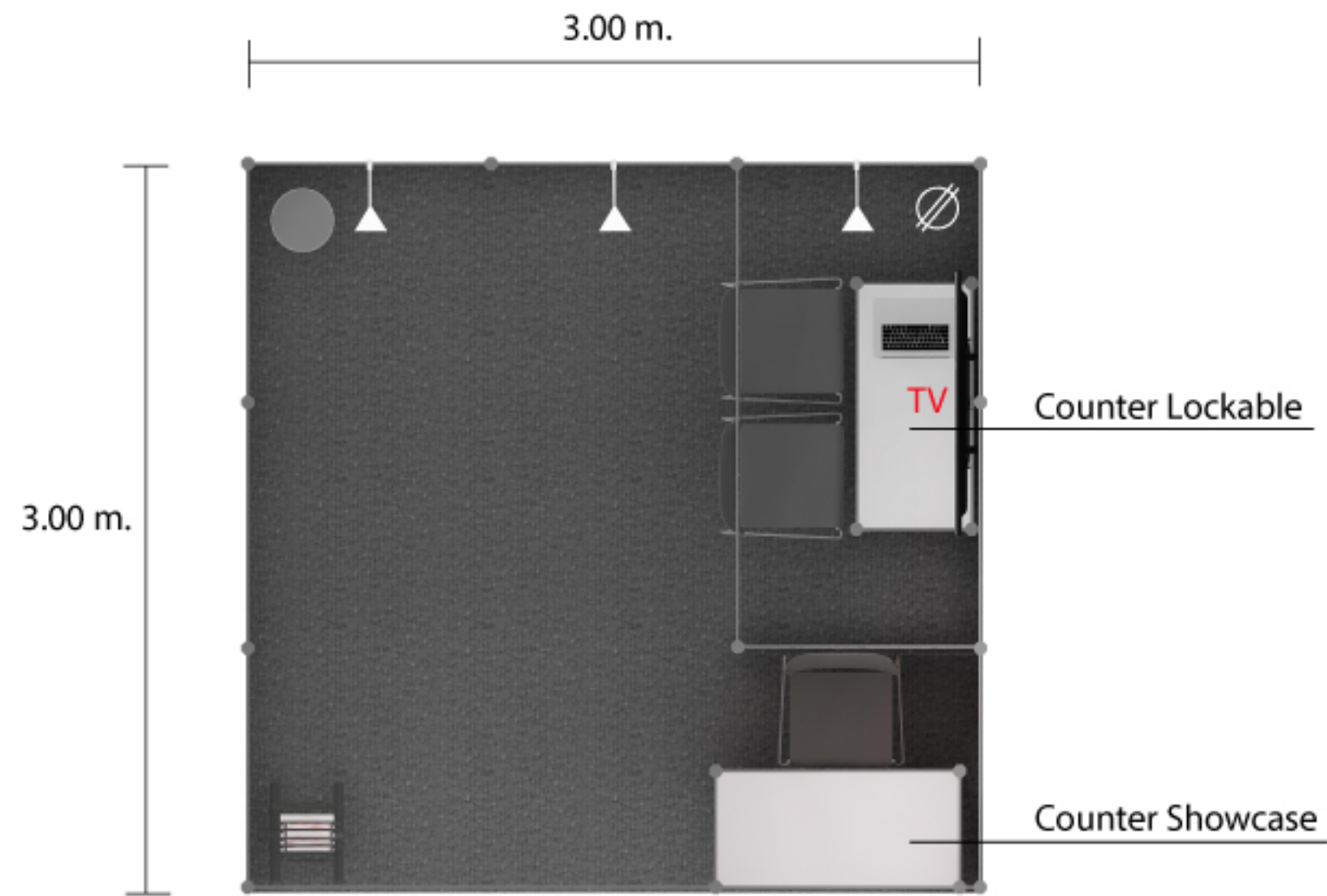
TOP VIEW
