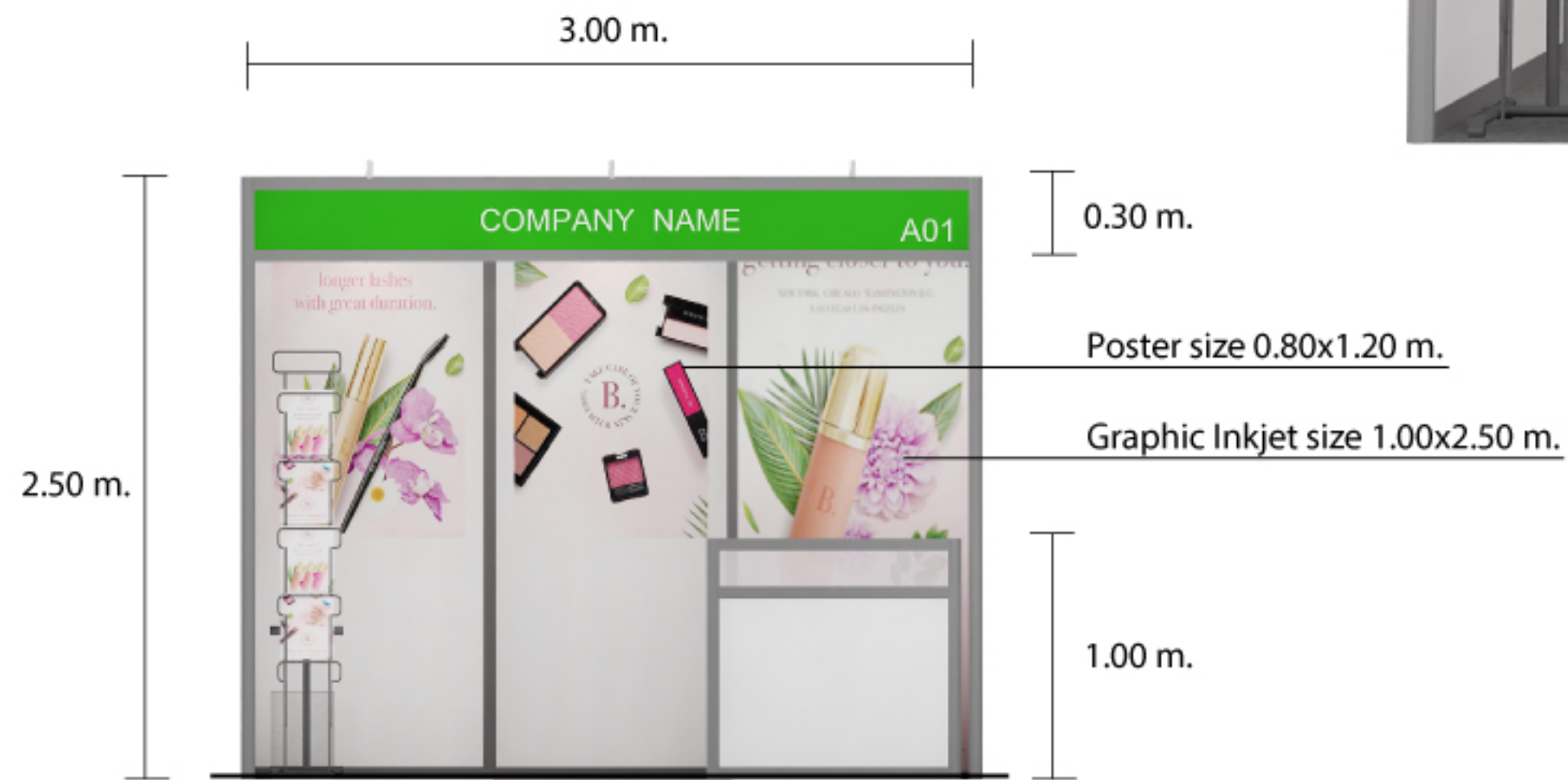
FRONT VIEW
