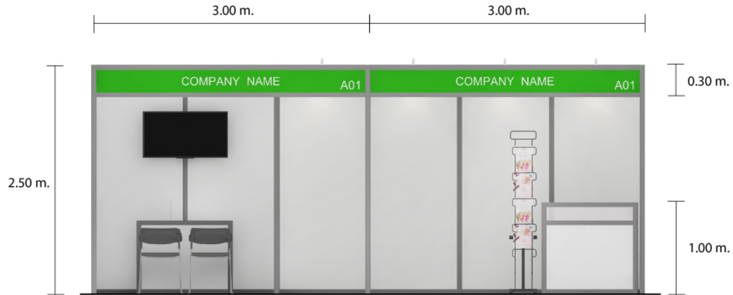
FRONT VIEW
